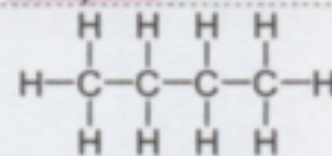
Figure 2. Butane Chemical Structure
