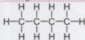
Figure 1. Propane Chemical Structure
