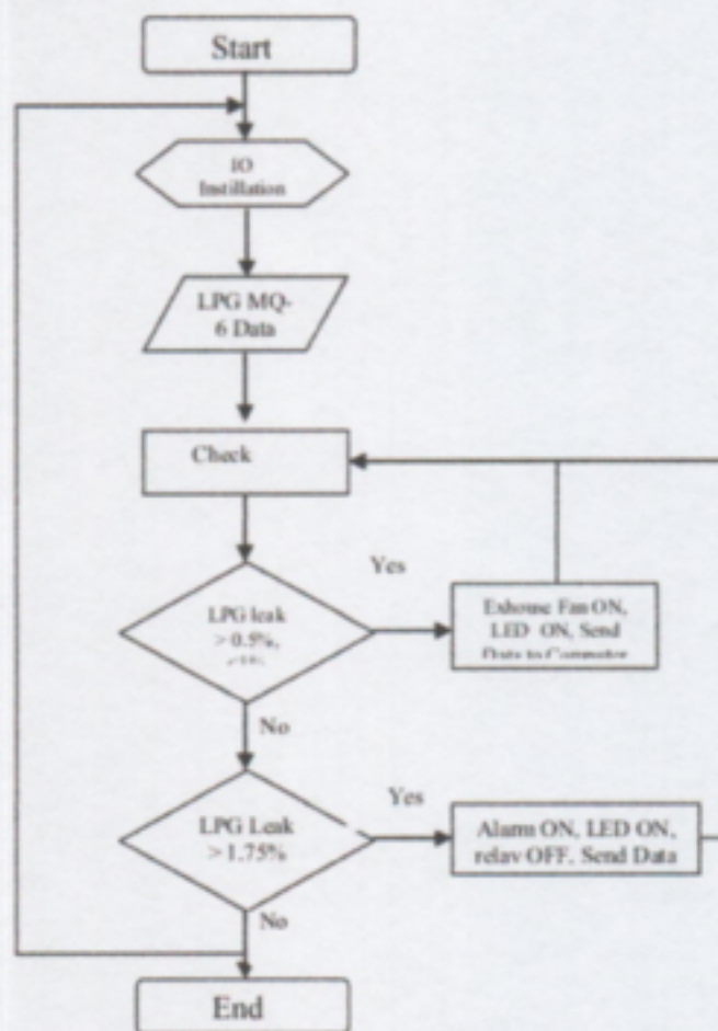
Figure 8. Software Design
