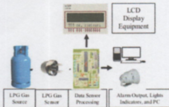
Figure 9. LPG Gas Detection Groove
