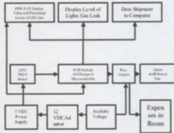
Figure 7. Flowchart Research
