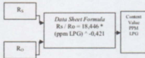
Figure 13. Sensor Calibration
